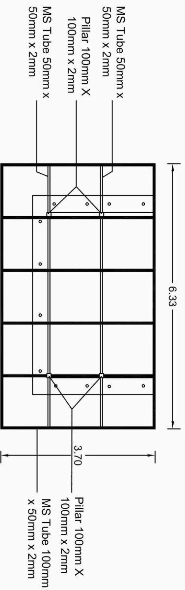
Balcony Plan 03
